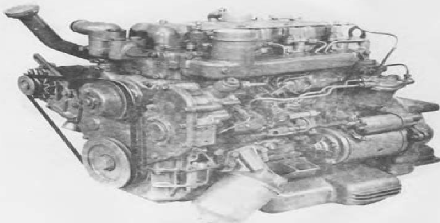
View of Front Left Hand Side of 4-154 Engine
