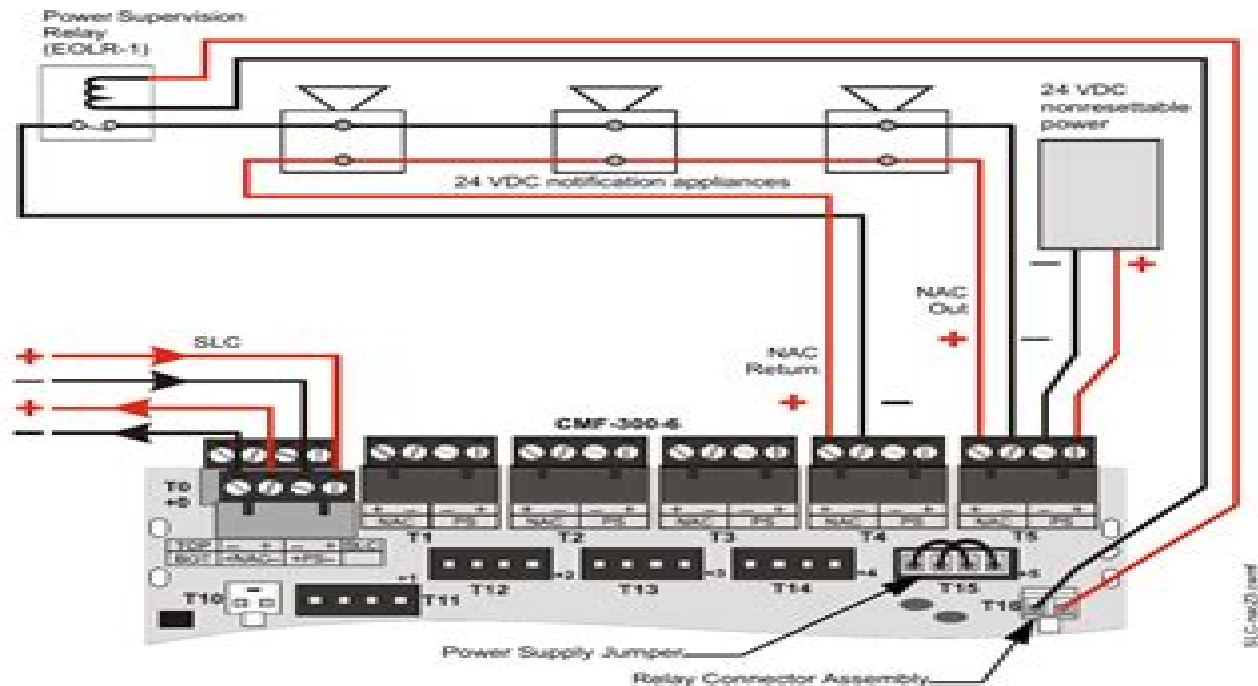
Figure 6.6 NFPA Style Z Notification Appliance Circuit
