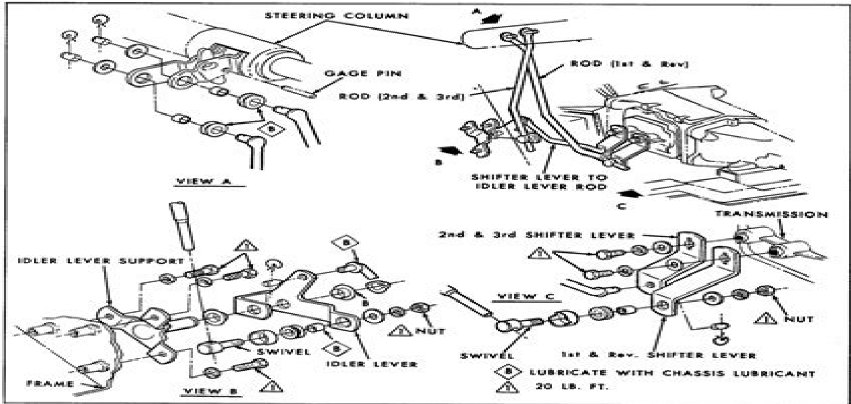
Fig. 7B-2 Firebird Column Shift Controls
