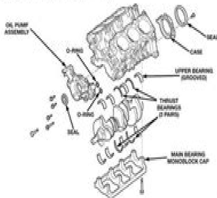
Fig. 16 Crankshaft and Cylinder Block
