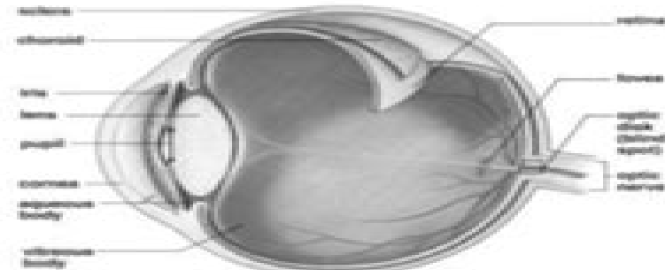
Fig. 32.39 Structure of the human eye.
