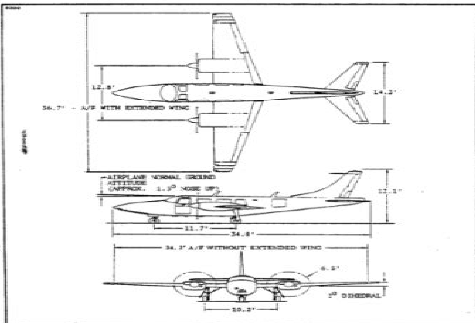
Figure 6-1. General Dimensions
