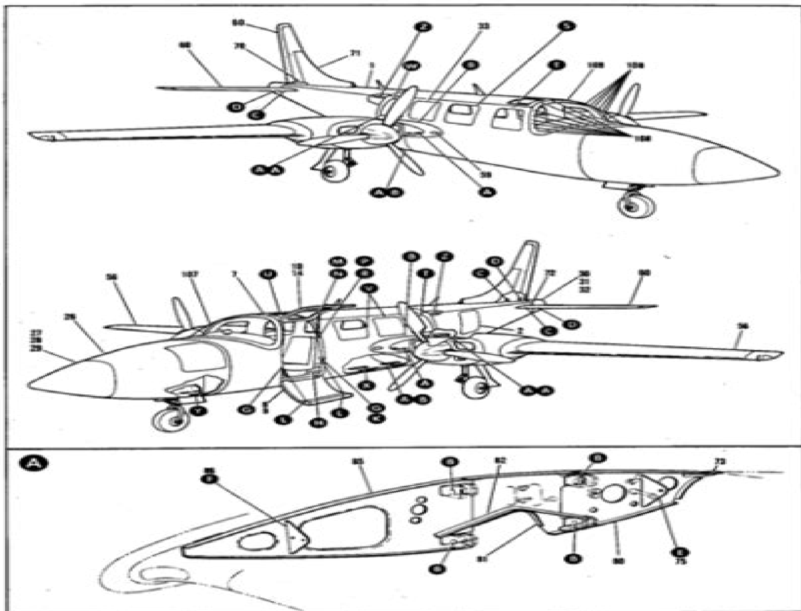
FIGURE 2-1. AIRPLANE COMPLETE (Sheet 1 of 7)
