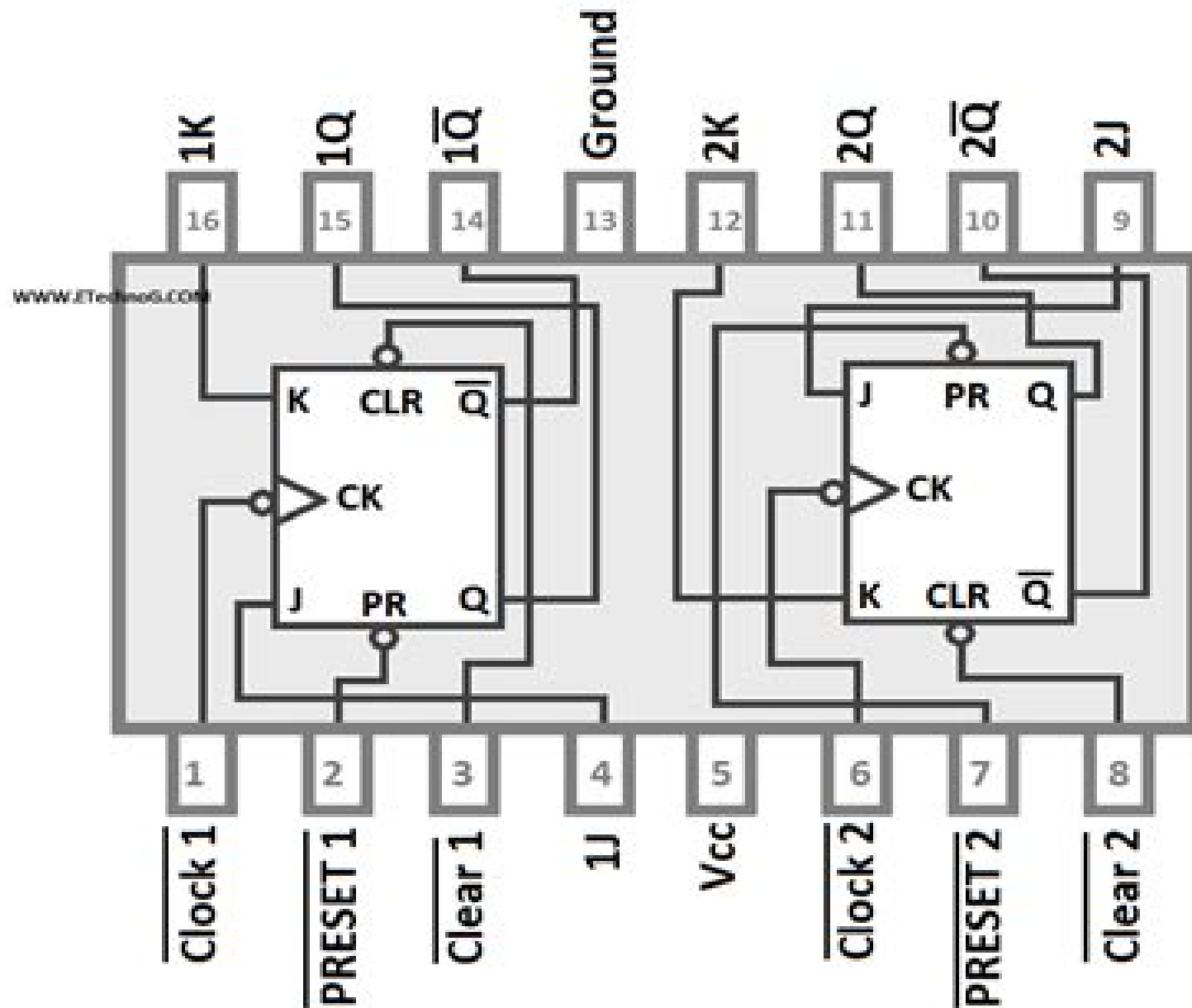
IC 7476 Pinout Diagram
