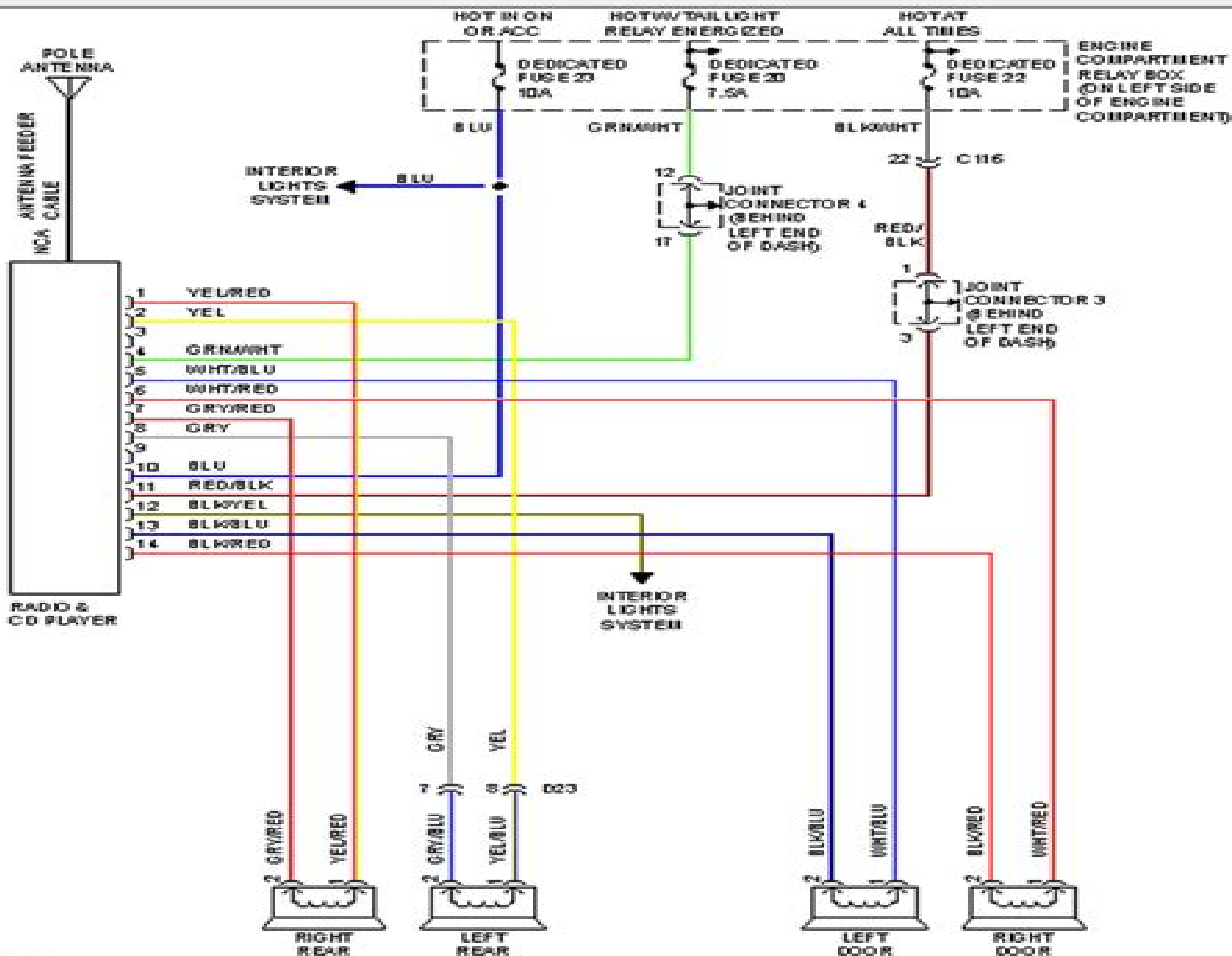
Fig. 39: Radio Circuit, W/D Amplifier
