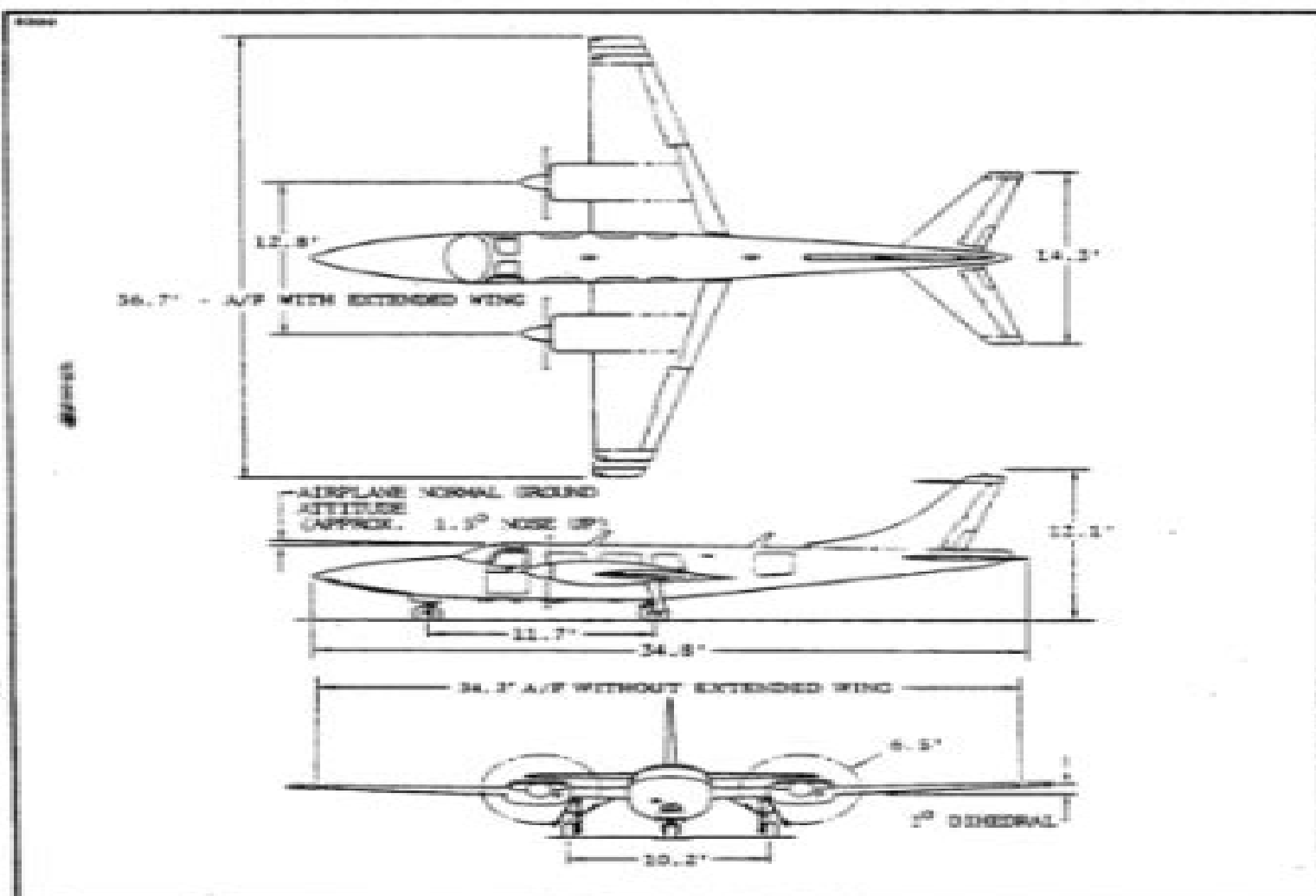
Figure 6-1. General Dimensions
