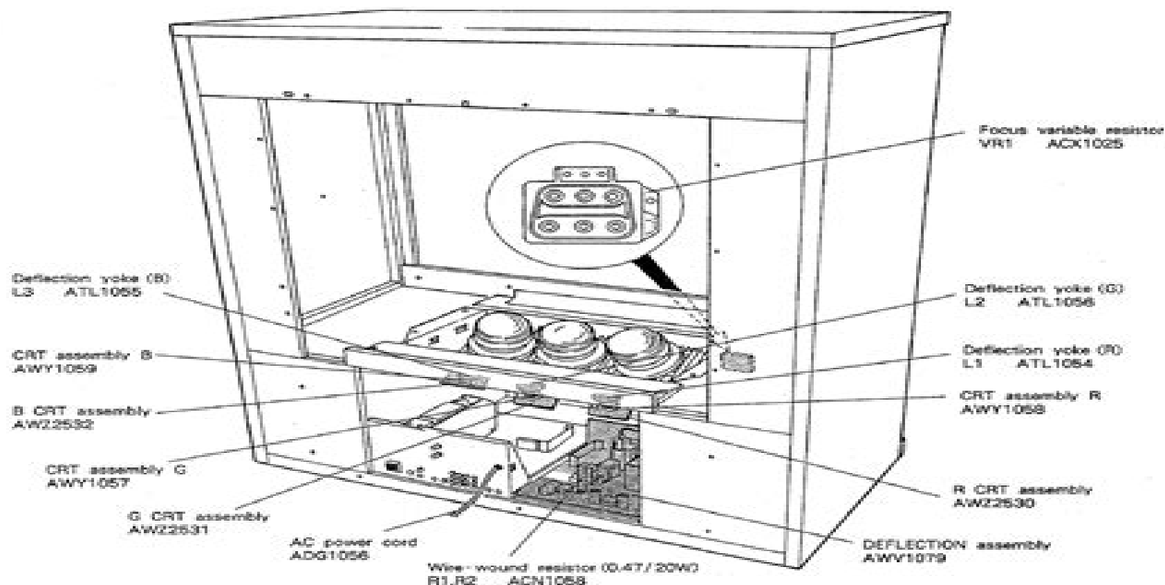
Fig. 3-1 Charged section and high voltage generating point
