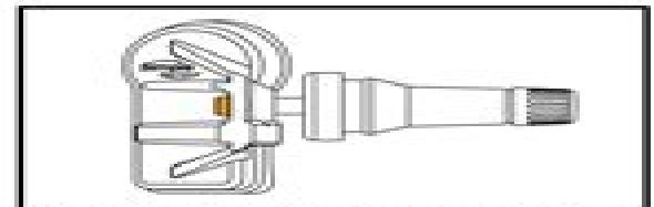
Step 1: Insert screw into valve stem tightly (1.5Nm)
