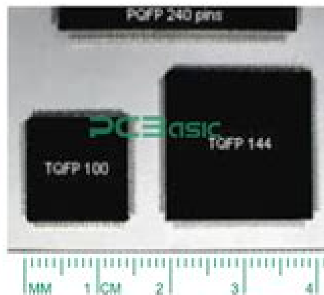
The Size of QFP
