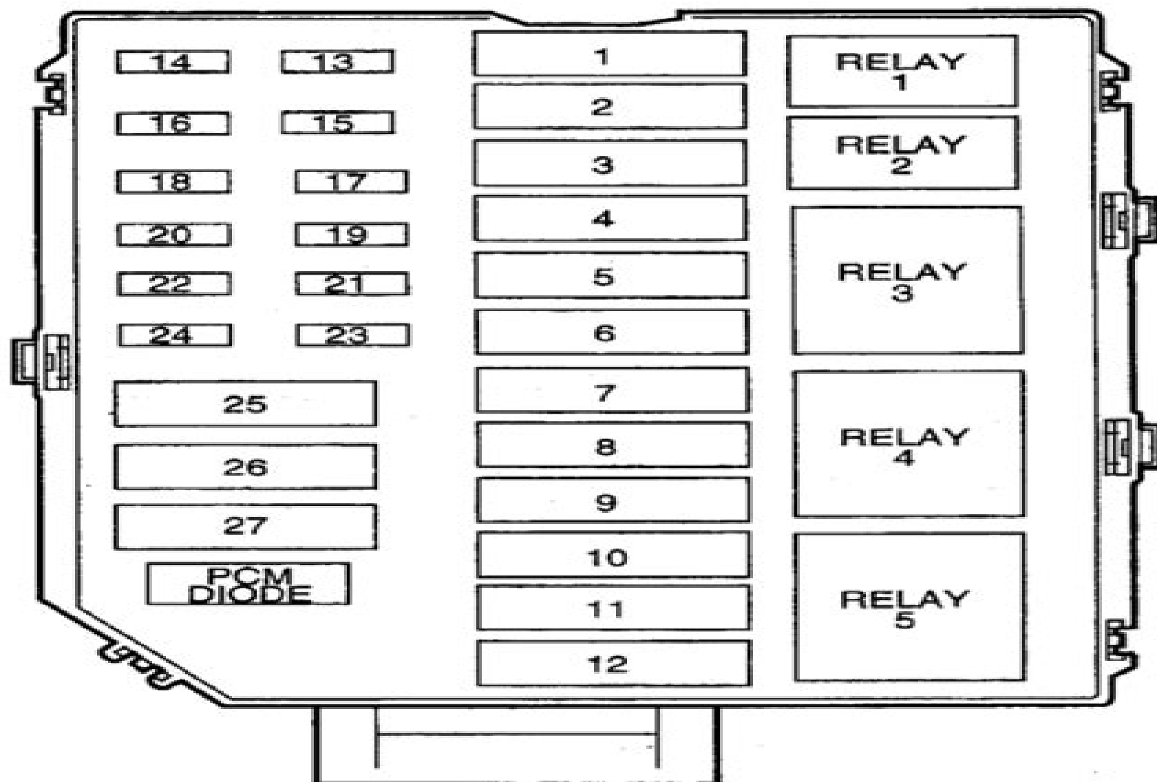
Fig 2: Identifying Battery Junction Box Components
