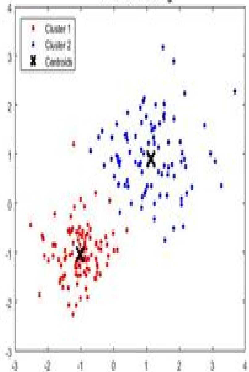
k-Means Clustering
