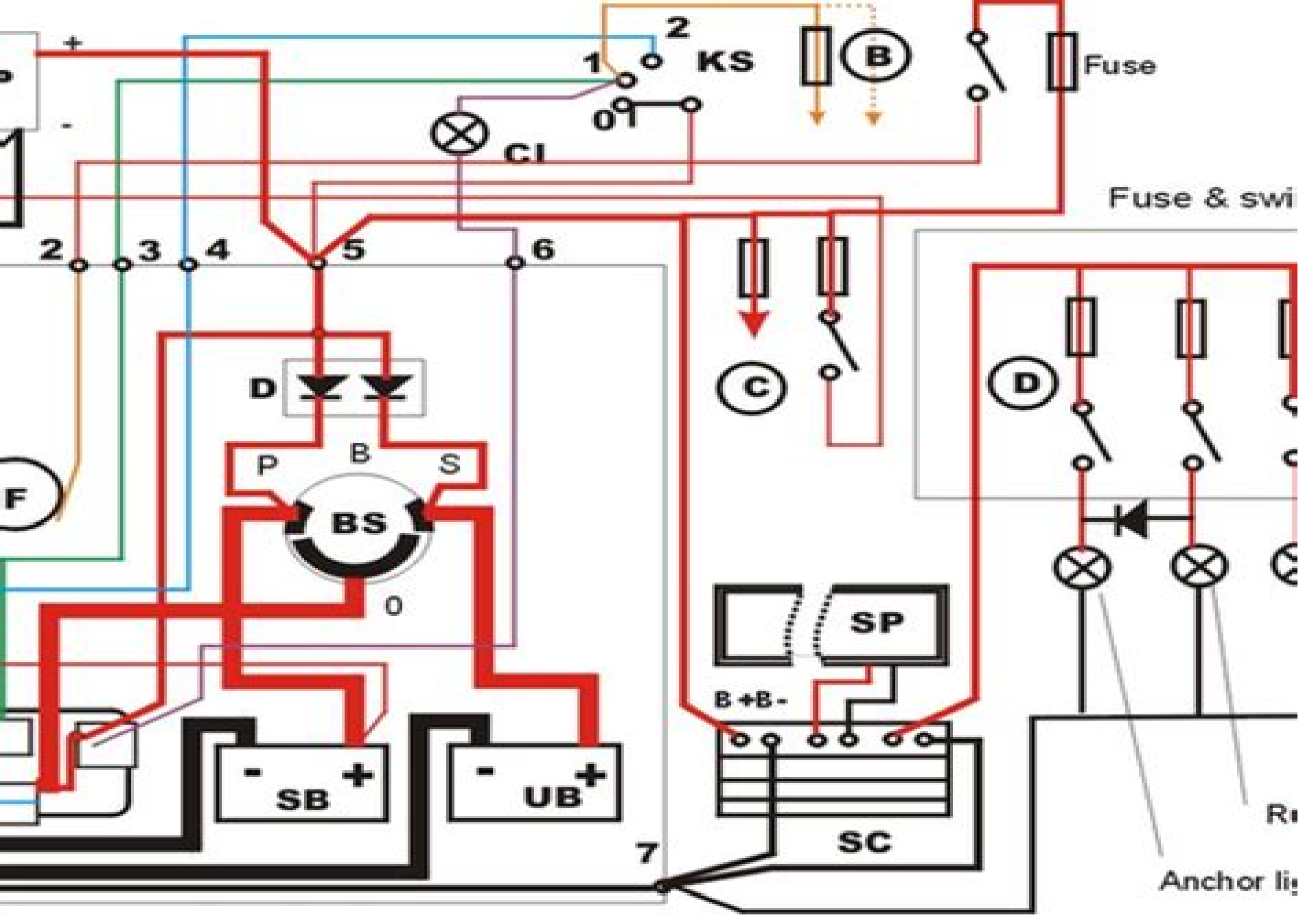
ical engine bay circuit
