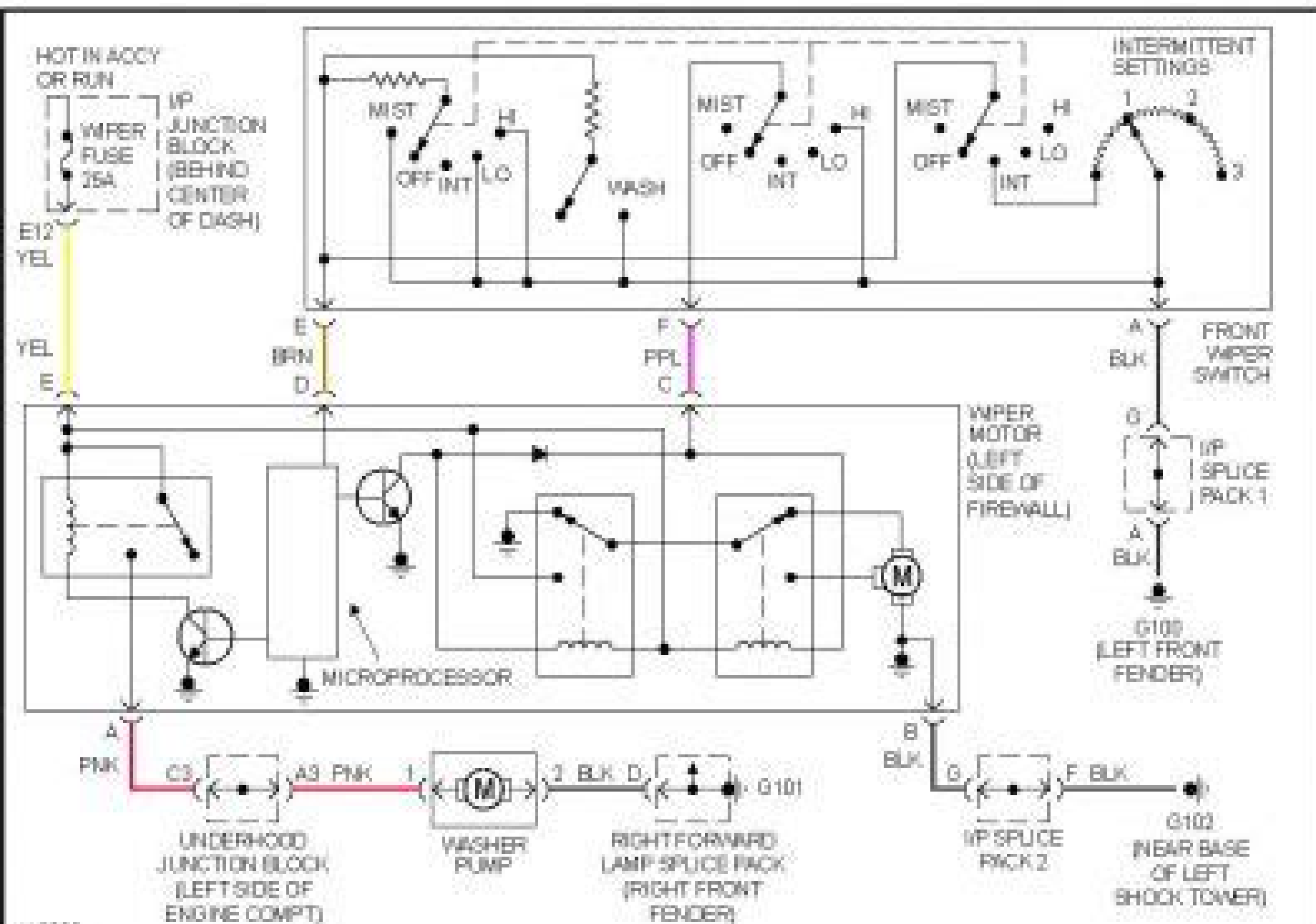
1999 Saturn SL1-Fig. 3: Front Wiper/Washer System Wiring Diagram (Saturn)
