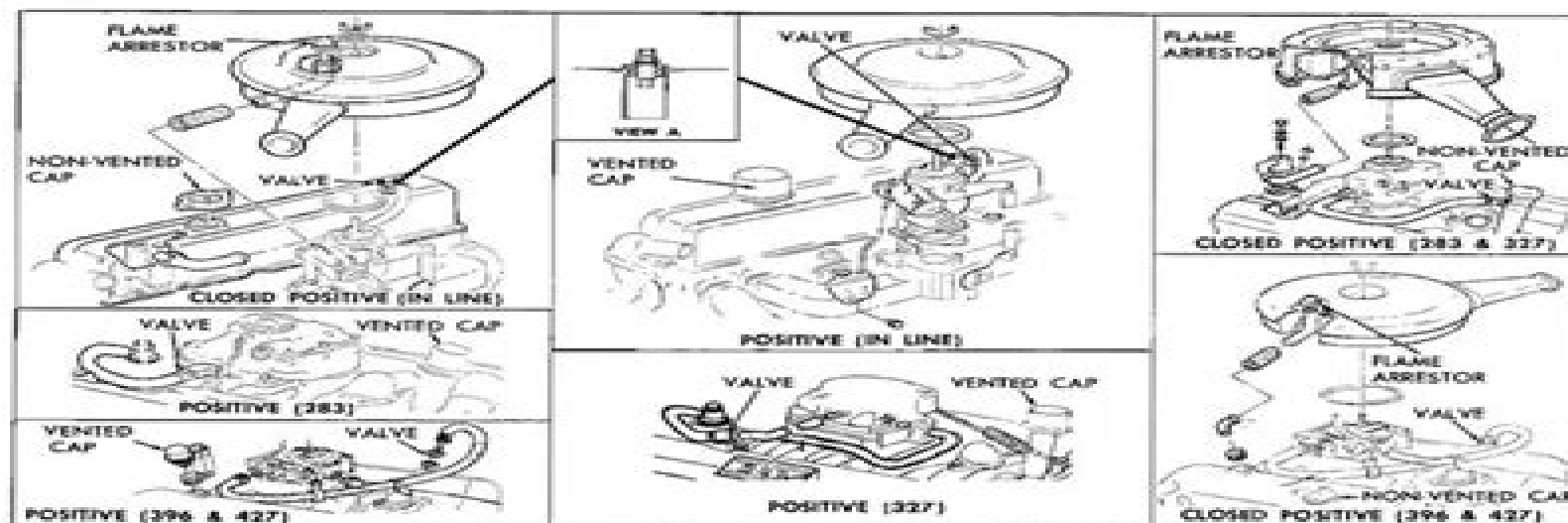
Fig. 10 - Crankcase Ventilation Systems
