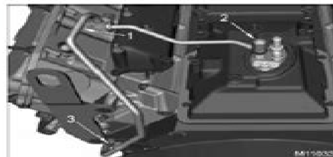
Figure 250 High-pressure pump to cooler tube assembly (upper connection)
