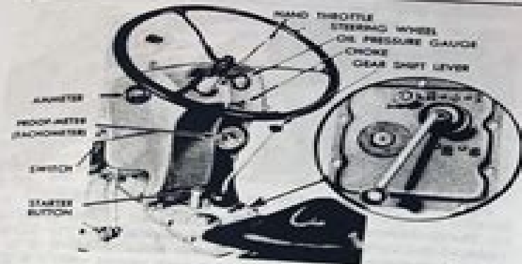
Fig. 5—Operator's Controls
