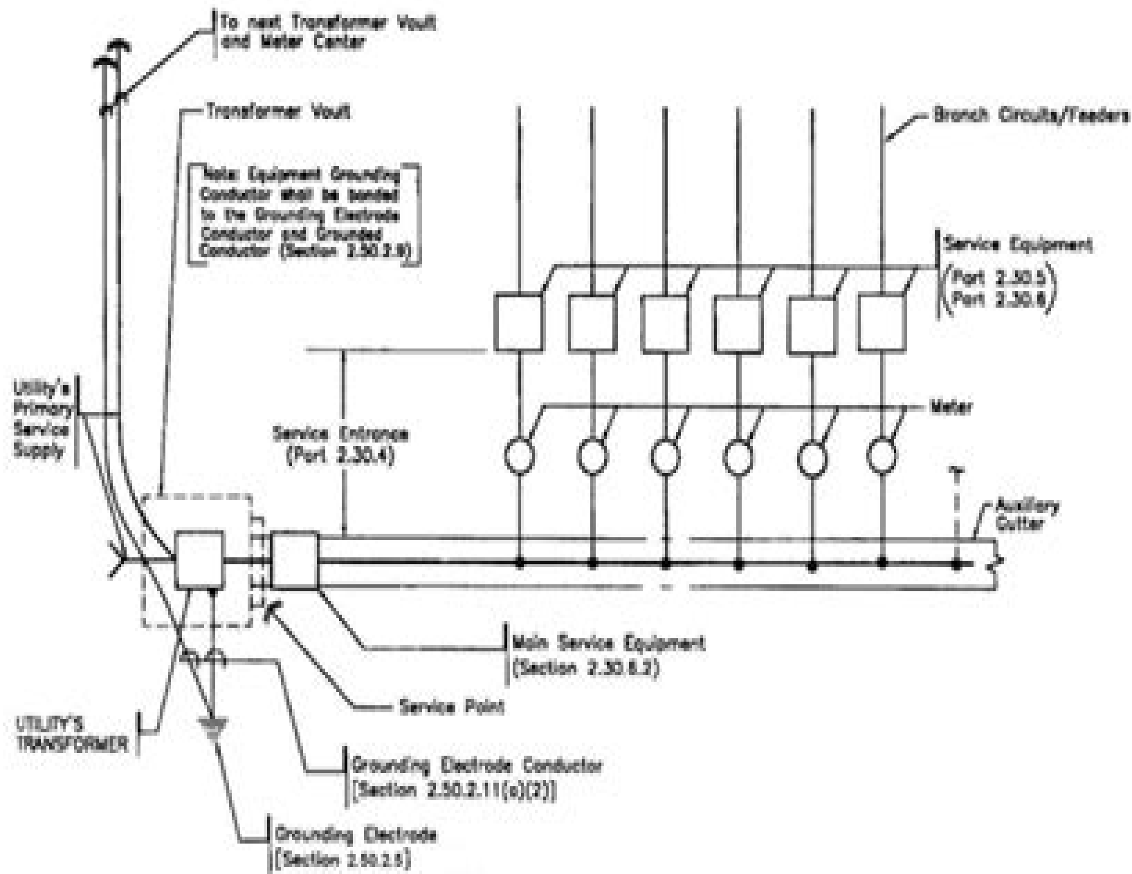
Figure 2.30.1.1(e) High Rise Building Services (not Exceeding 600 Volts), Multiple Occupancy
