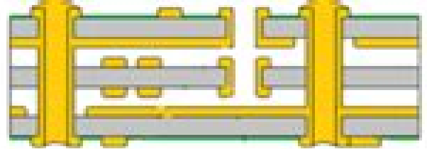
Multi-Layer PCB
