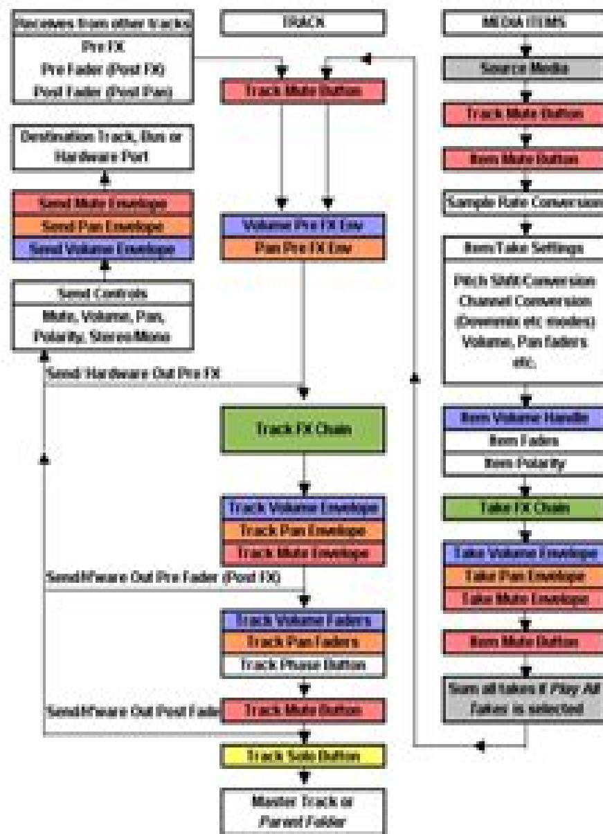
REAPER Audio Playback Signal Flow - Top Level Track or Child Track
