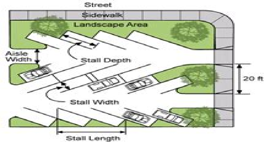
30-Degree Angle Parking
