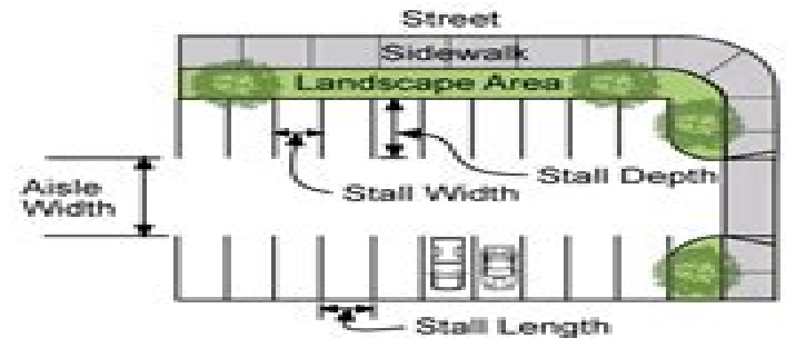
90-Degree Parking
