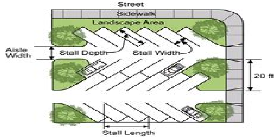
45-Degree Angle Parking
