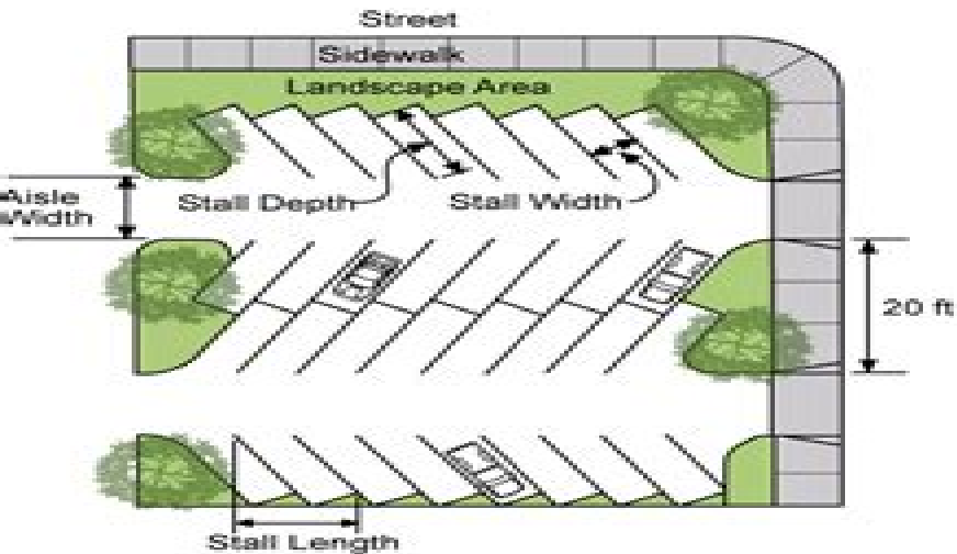
60-Degree Angle Parking
