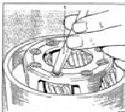
Fig. 11B-14 Staking a piston pin 1. Circlip
