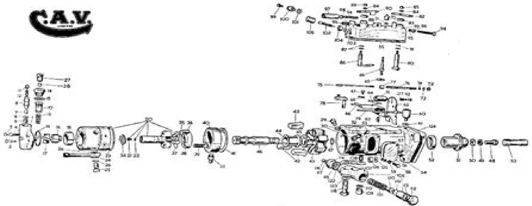
Mechanically Governed CAV DPA pump
