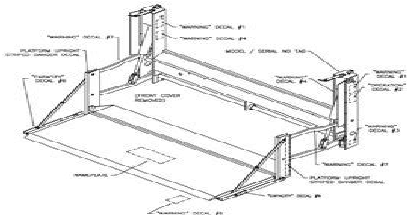
Figure 9 – Decal Location Diagram
