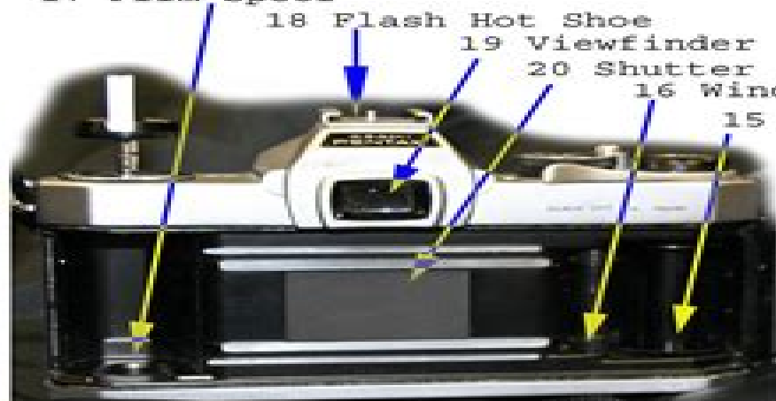
Manual SLR Film Camera Parts
