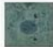
Entamoeba nana
