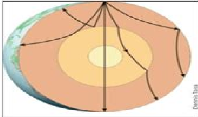
Figure 14 The arrows show only a few of the many possible paths that seismic waves take through Earth. Inferring What causes the wave paths to change?
