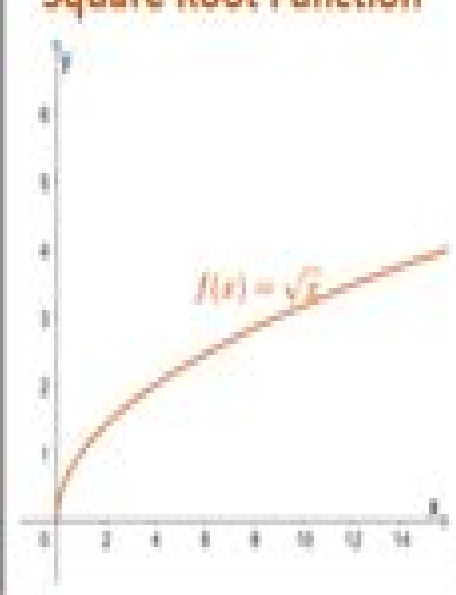
Square Root Function
