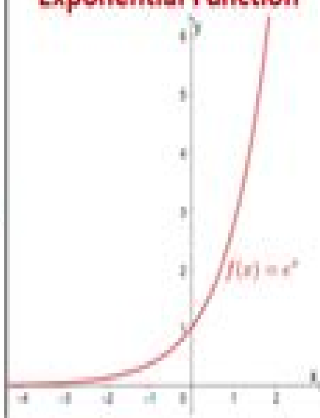
Exponential Function
