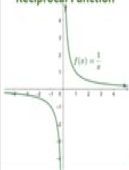
Reciprocal Function
