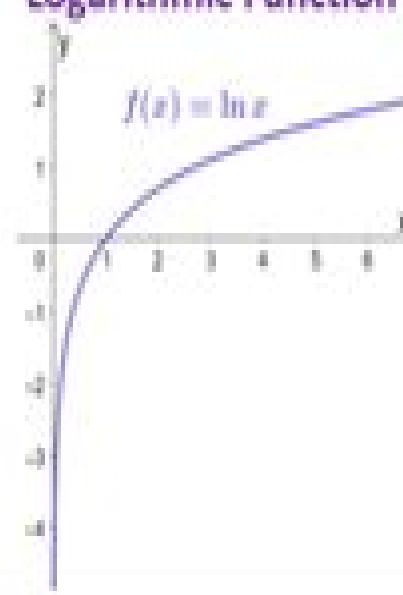
Logarithmic Function
