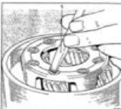
Fig. 11B-14 Staking a piston pin 1. Check
