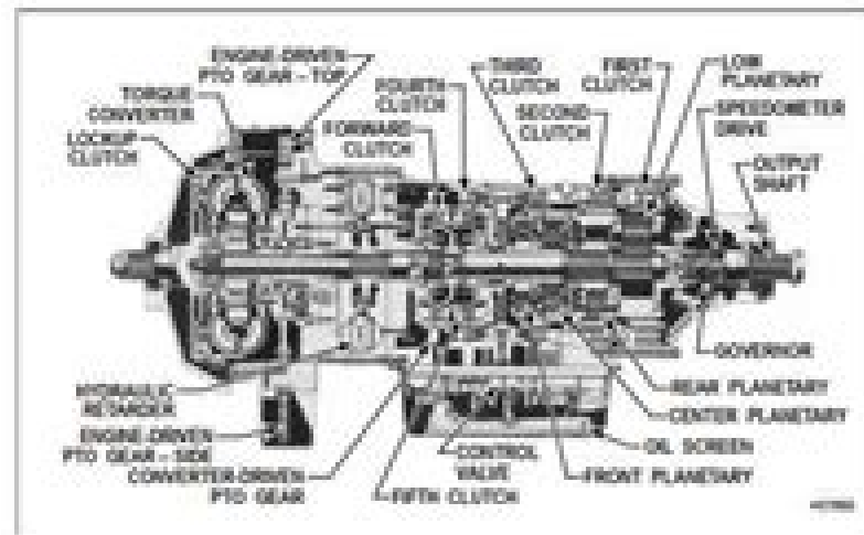
Figure 3. CLBT 750/754 Remote Mount—Cross Section
