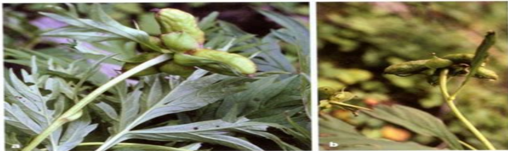
Fig. 3.10. Polymorphism in indumentum on follicles in P. anomala subsp. tschuii in the population Hong et al. 1195034 (Lixian, Sichuan Province): a , glabrous; b , sparsely hairy.
