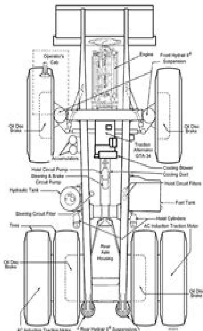
800E MAJOR COMPONENTS
