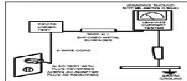
Figure 1-1. Leakage Current Test Circuit
