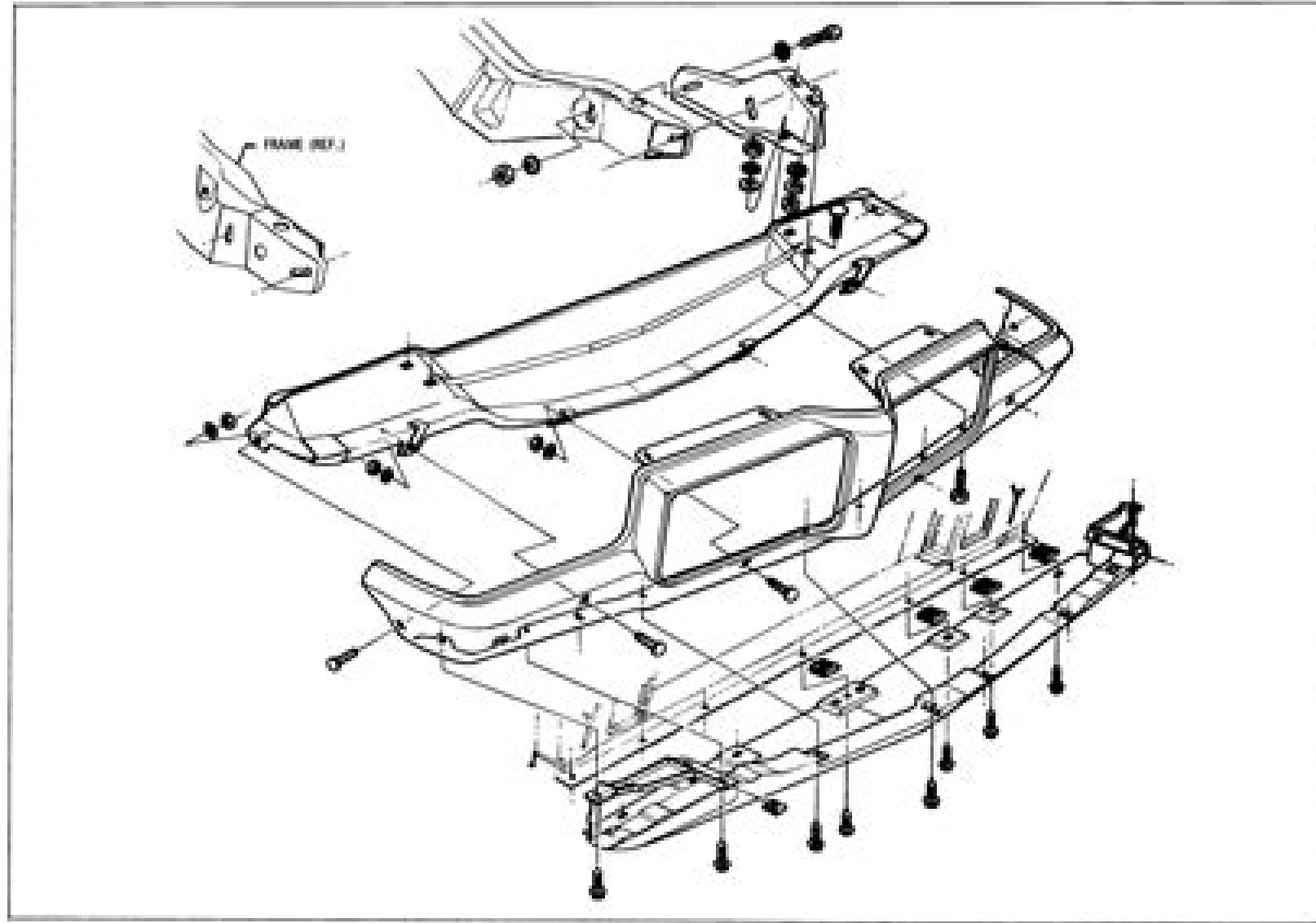
Fig. 14-7 Tempest Front Bumper and Valance Panel
