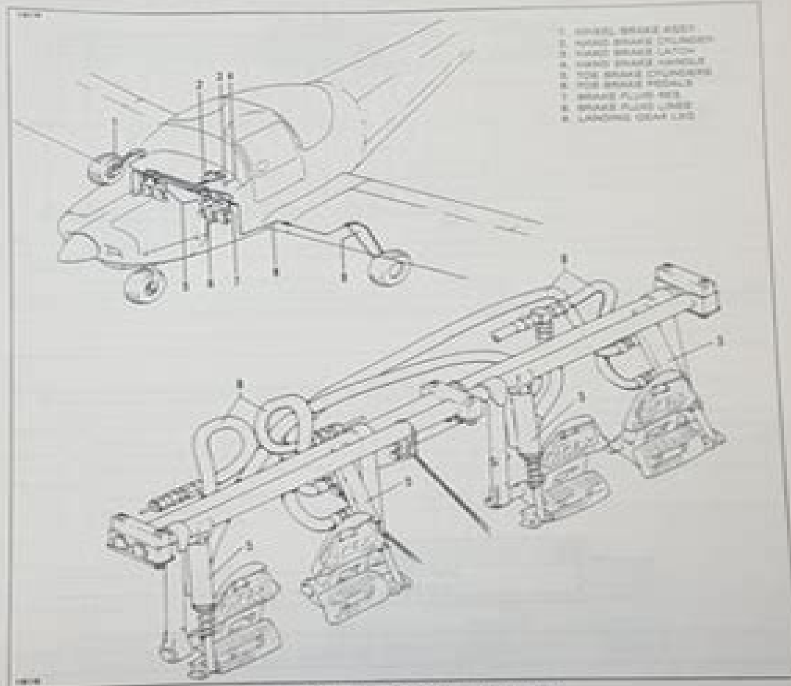
Figure 32-9. Toe Brake System Installation
