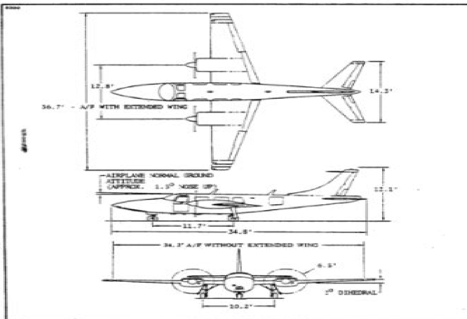
Figure 6-1. General Dimensions
