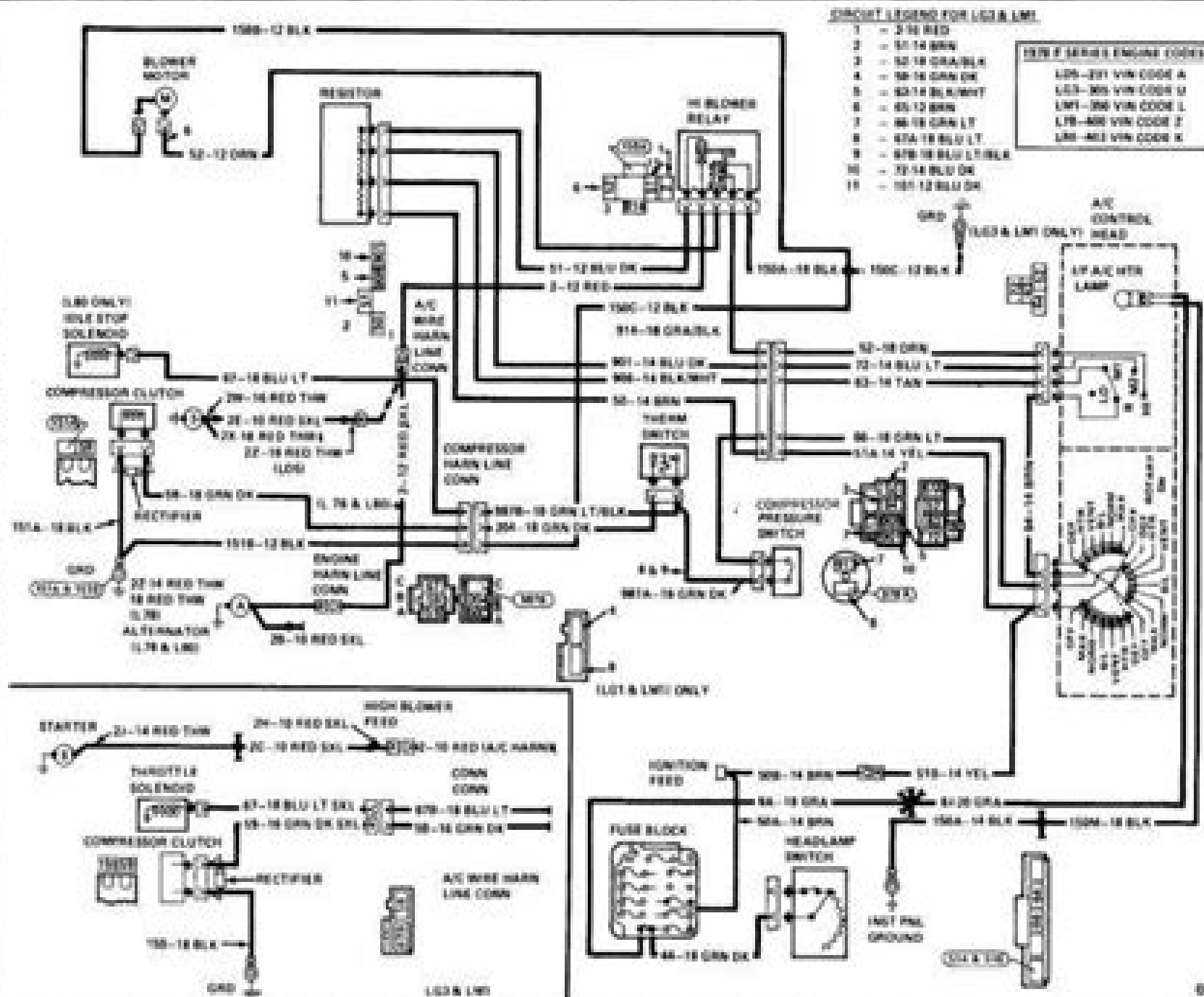
Fig. 1B-4 1978 F Series C60 A/C Wiring
