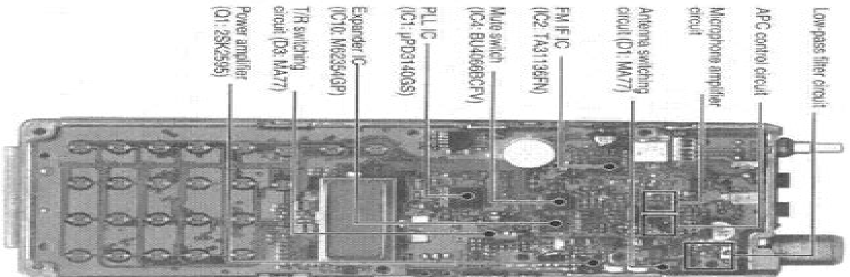
TOP VIEW
