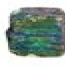
rainbow pyrite
