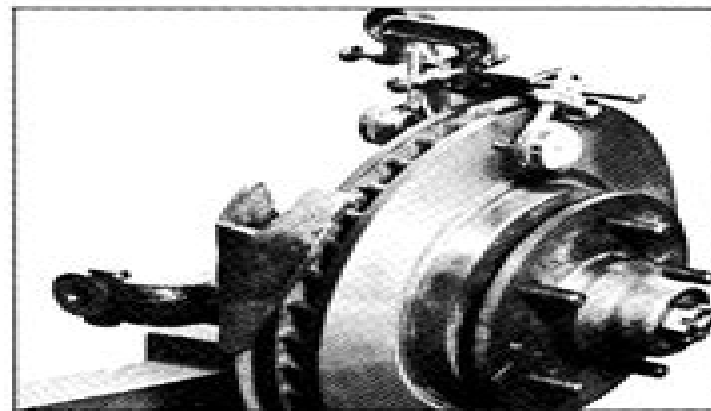
Fig. 5E-17 Measuring Parallelism
