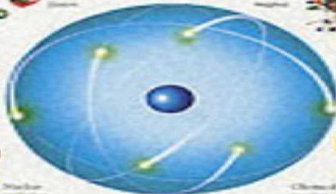
Atom
