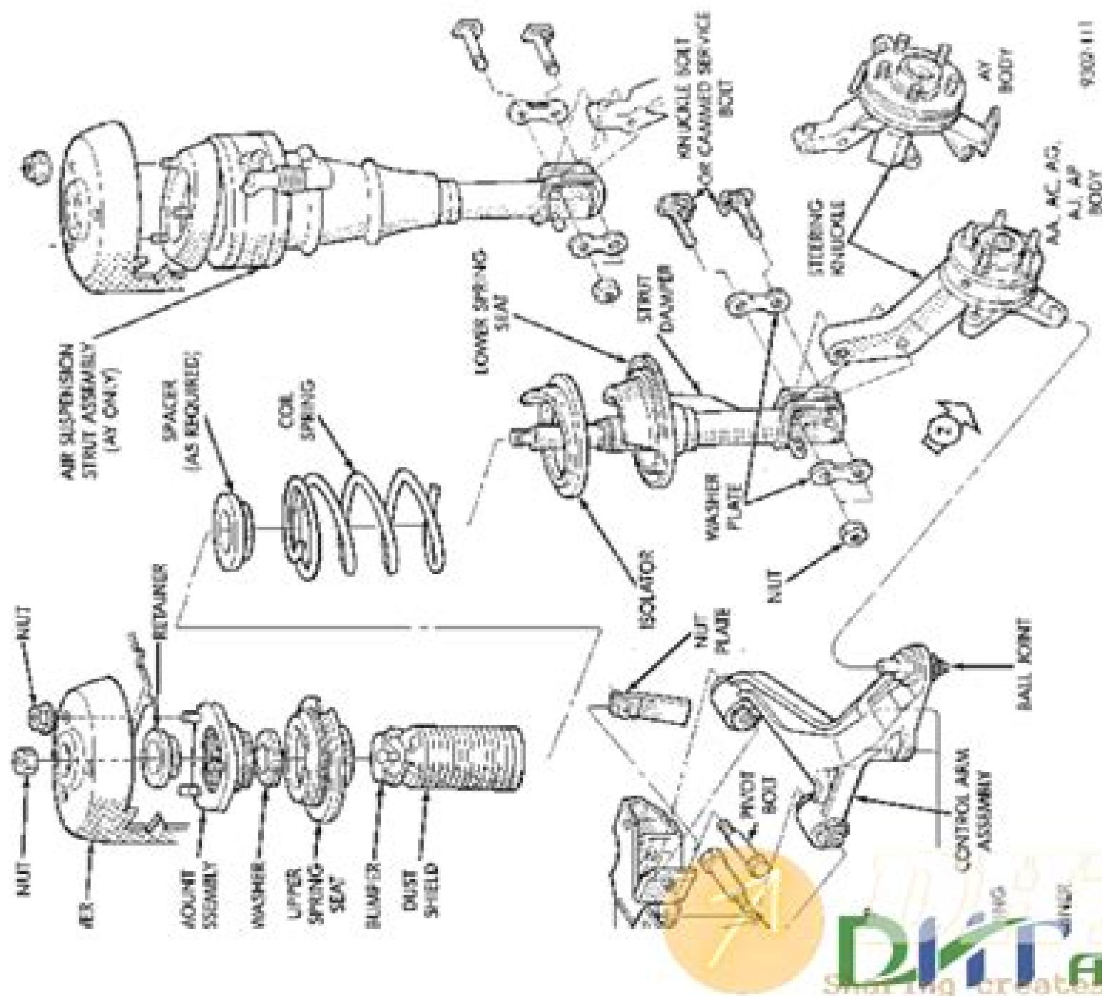
Fig. 2 Front Suspension Components
