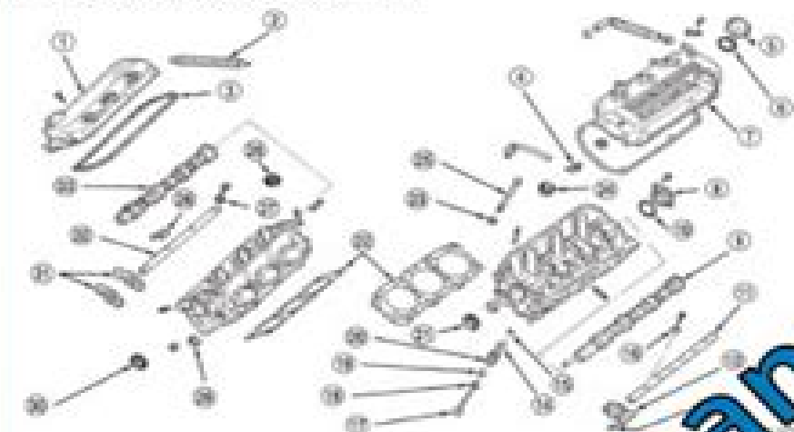
Fig. 4 Cylinder Head and Valve Train
