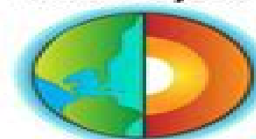
Earth Layers
