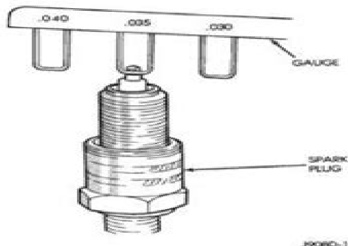
Fig. 6 Setting Spark Plug Electrode Gap—Typical
