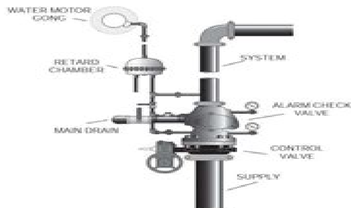
Figure 1-6 Typical Alarm Check Valve Riser
