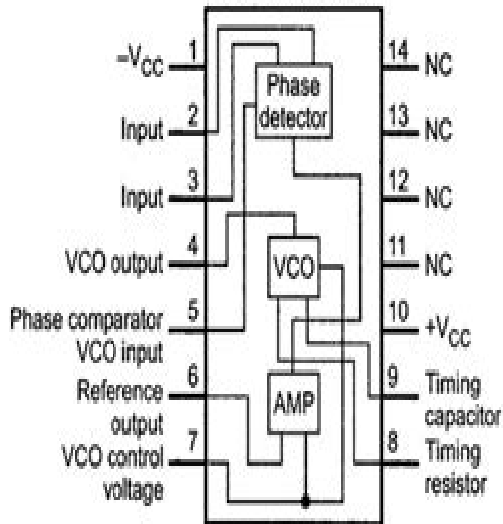
Dual-in-line package
